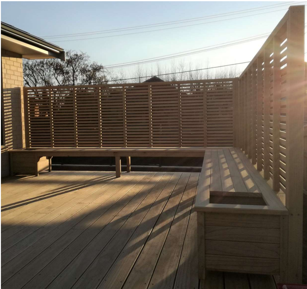
Trellis fencing in combination with bench seating and planters
