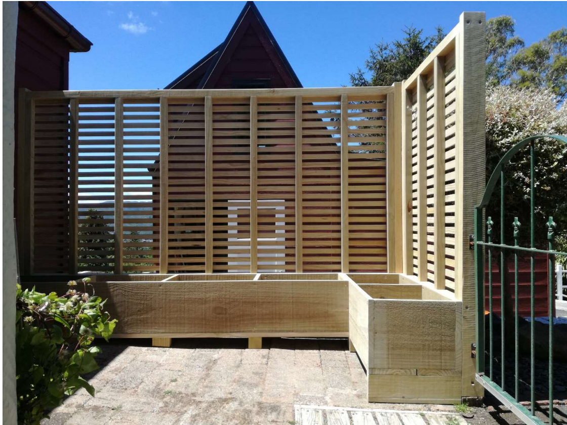
Corner trellis and planter unit built insitu
